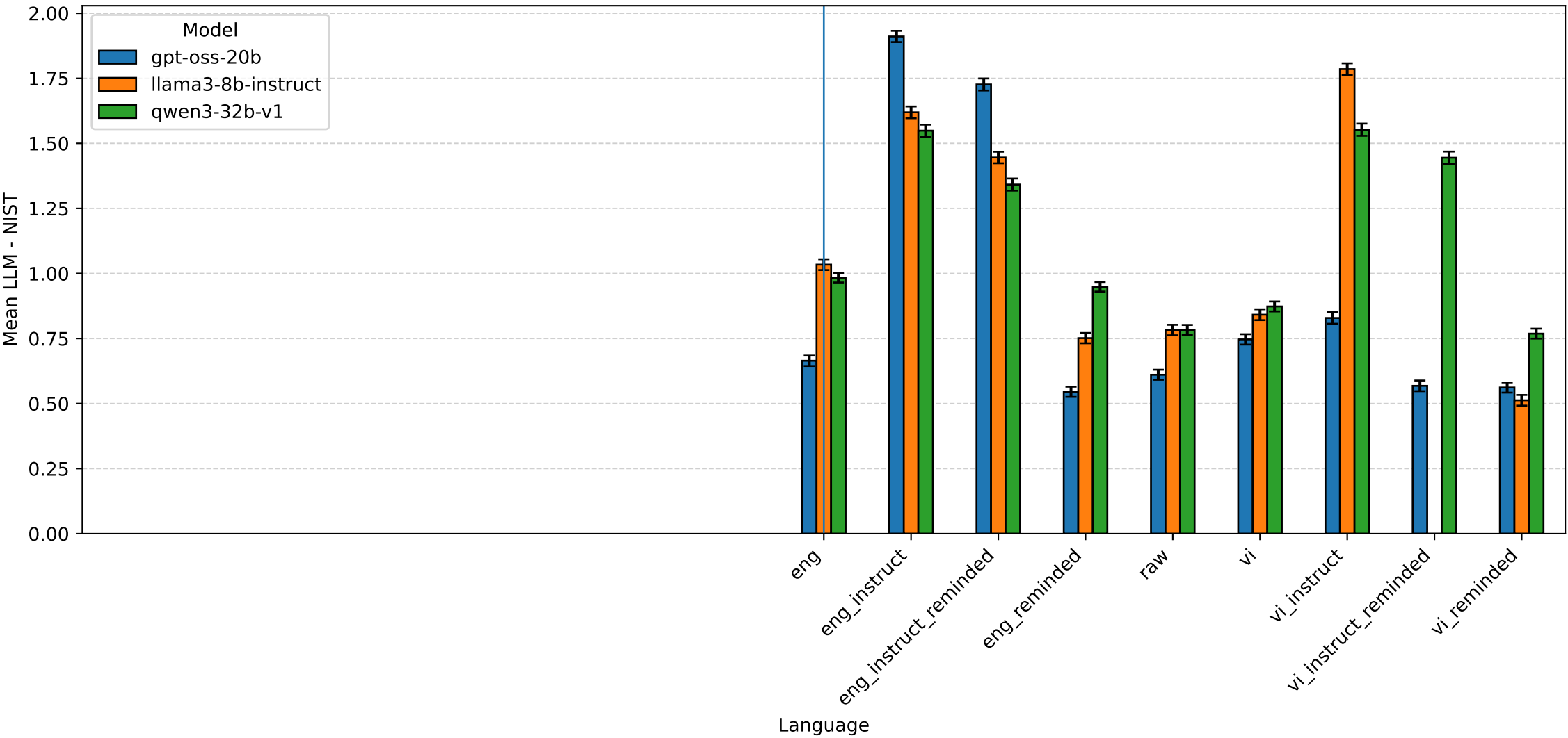
Mean relevance inflation by language and model (2021)
