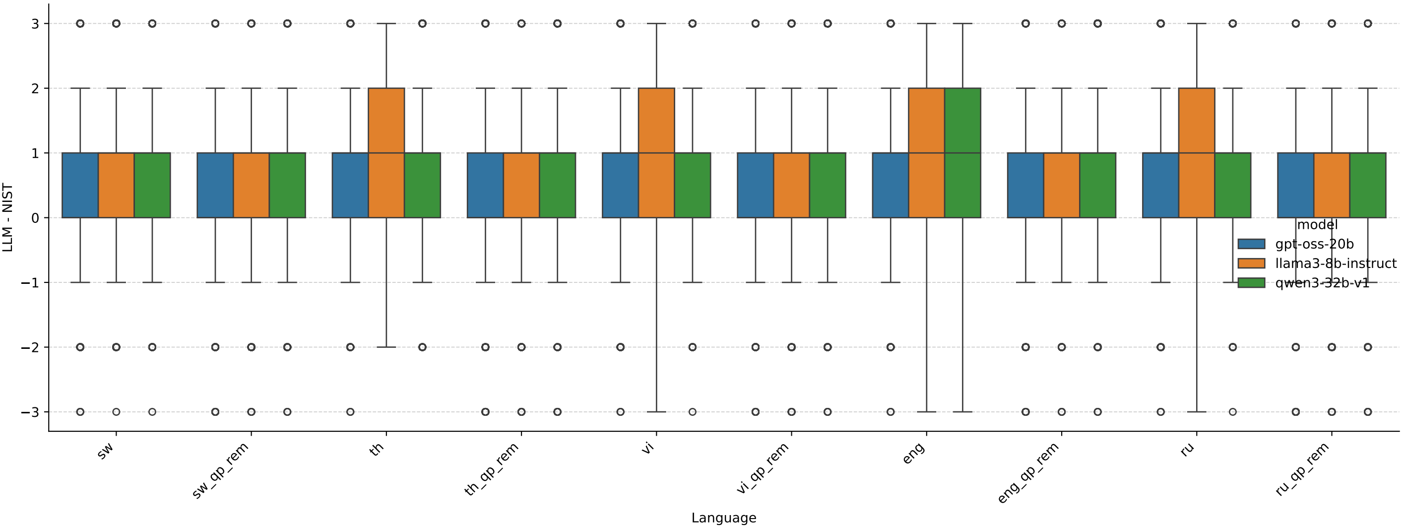
Distribution of relevance inflation by language and model, 2021-2022
