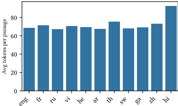
TREC-DL 2021 • Profile: lang
