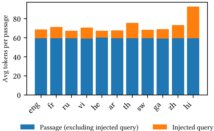
TREC-DL 2021 • Profile: lang • Query share in passage
