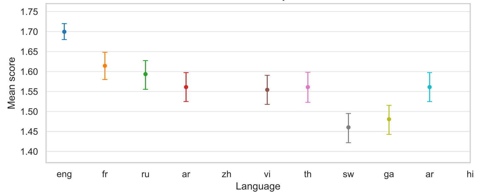
Contextuality
