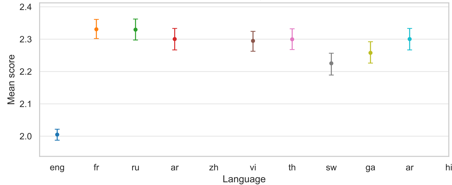
Exactness
