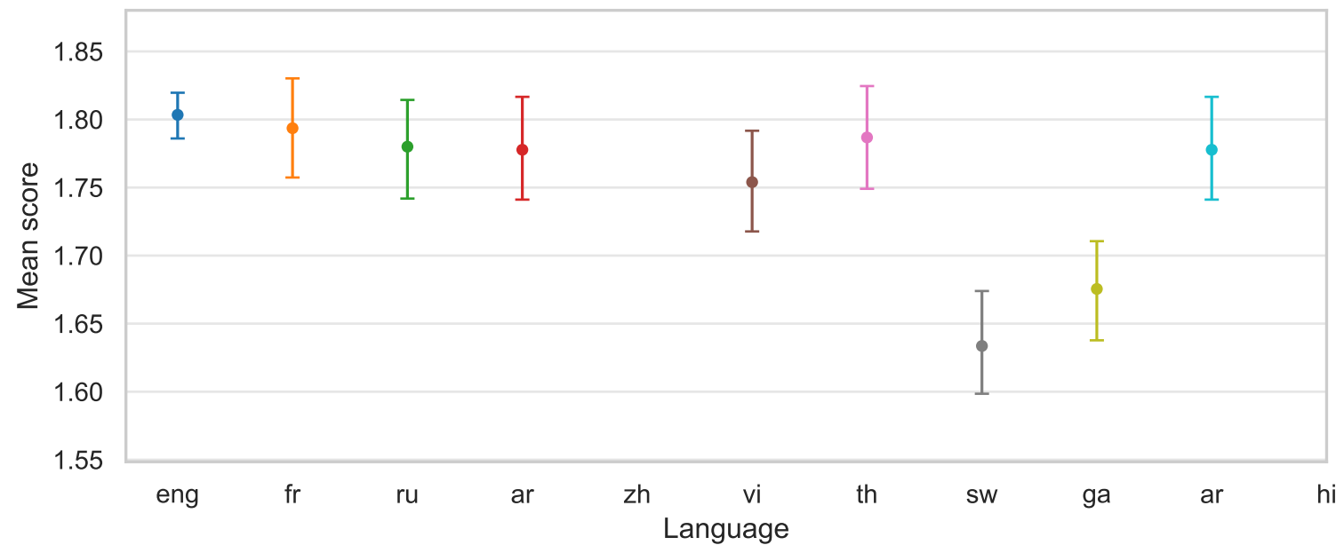
Exactness
