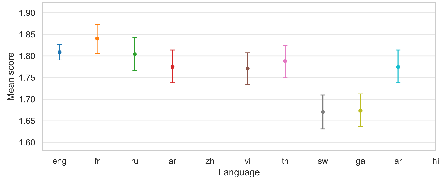
Contextuality
