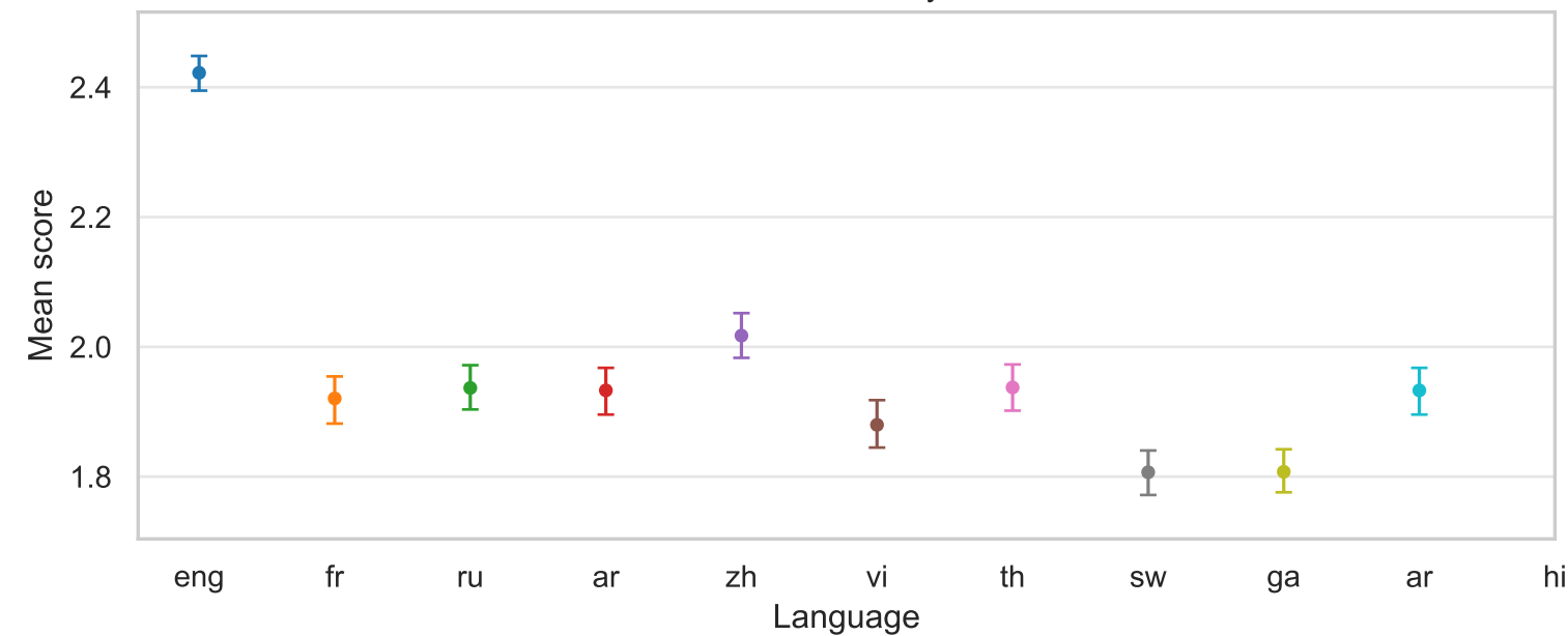
Contextuality
