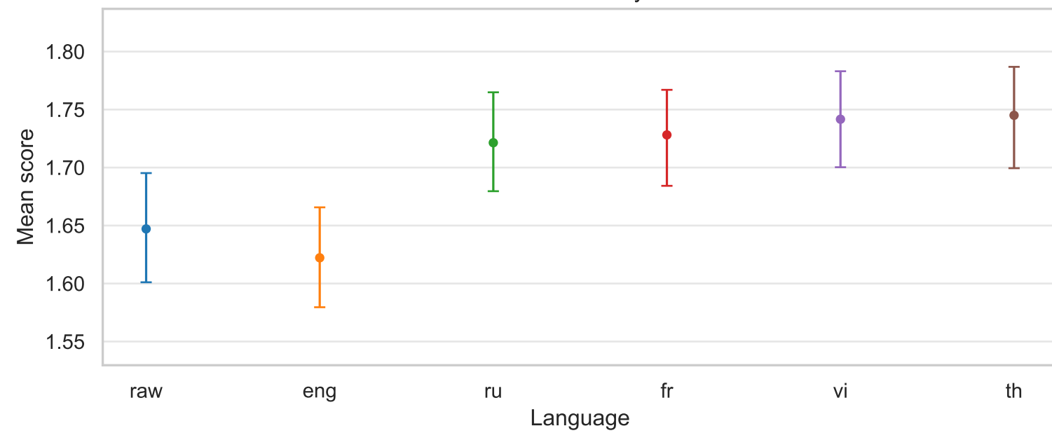
Contextuality
