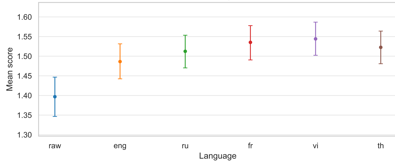
Contextuality
