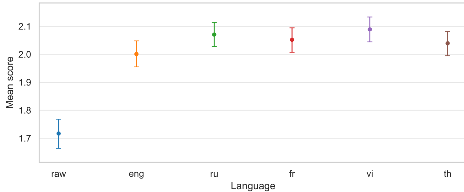
Exactness
