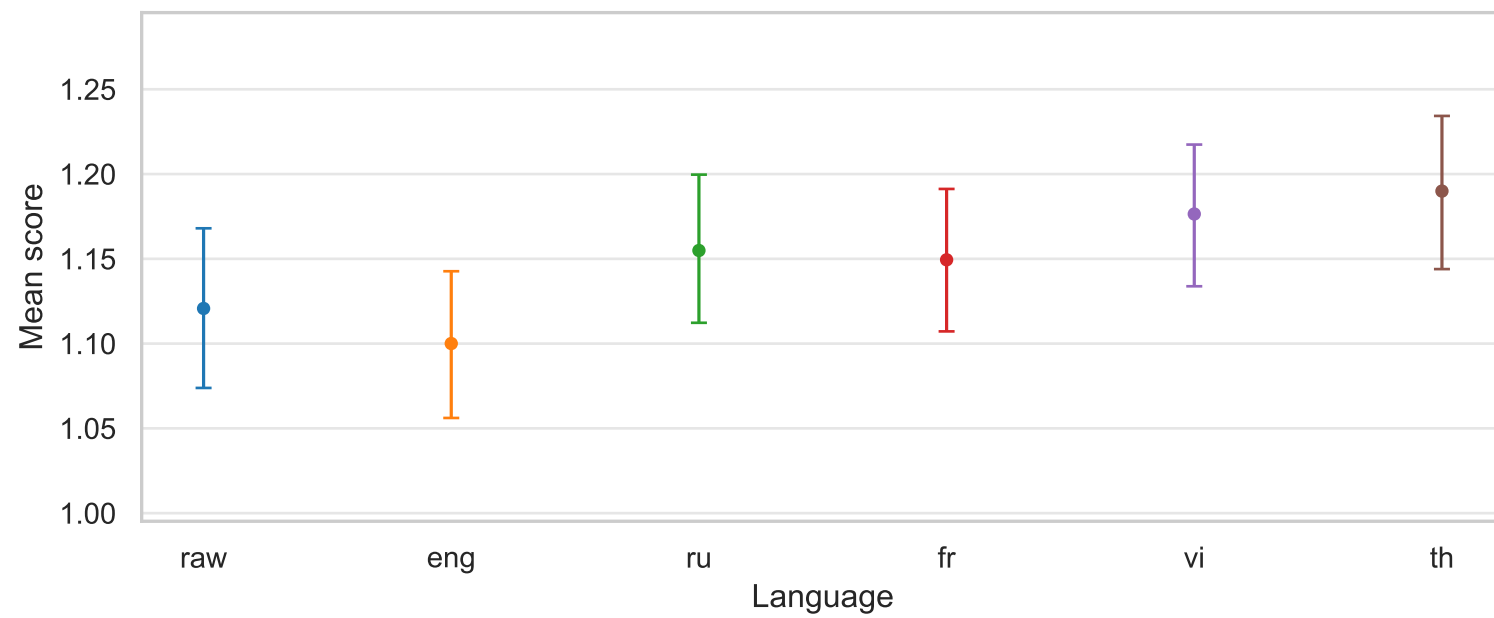
Exactness
