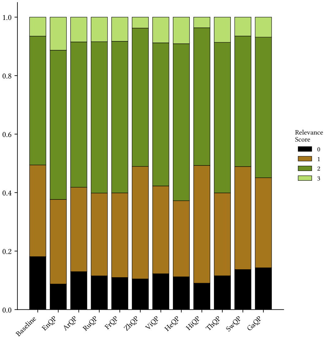
Relevance Label Score Distribution
