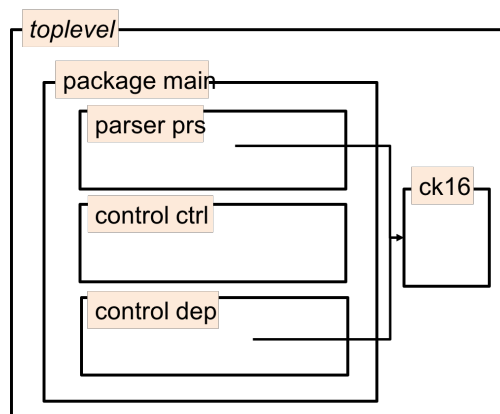
Figure 8. Evaluation result.
