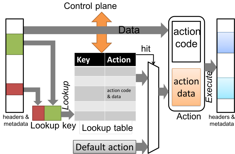
Figure 12. Match-Action Unit Dataflow.
