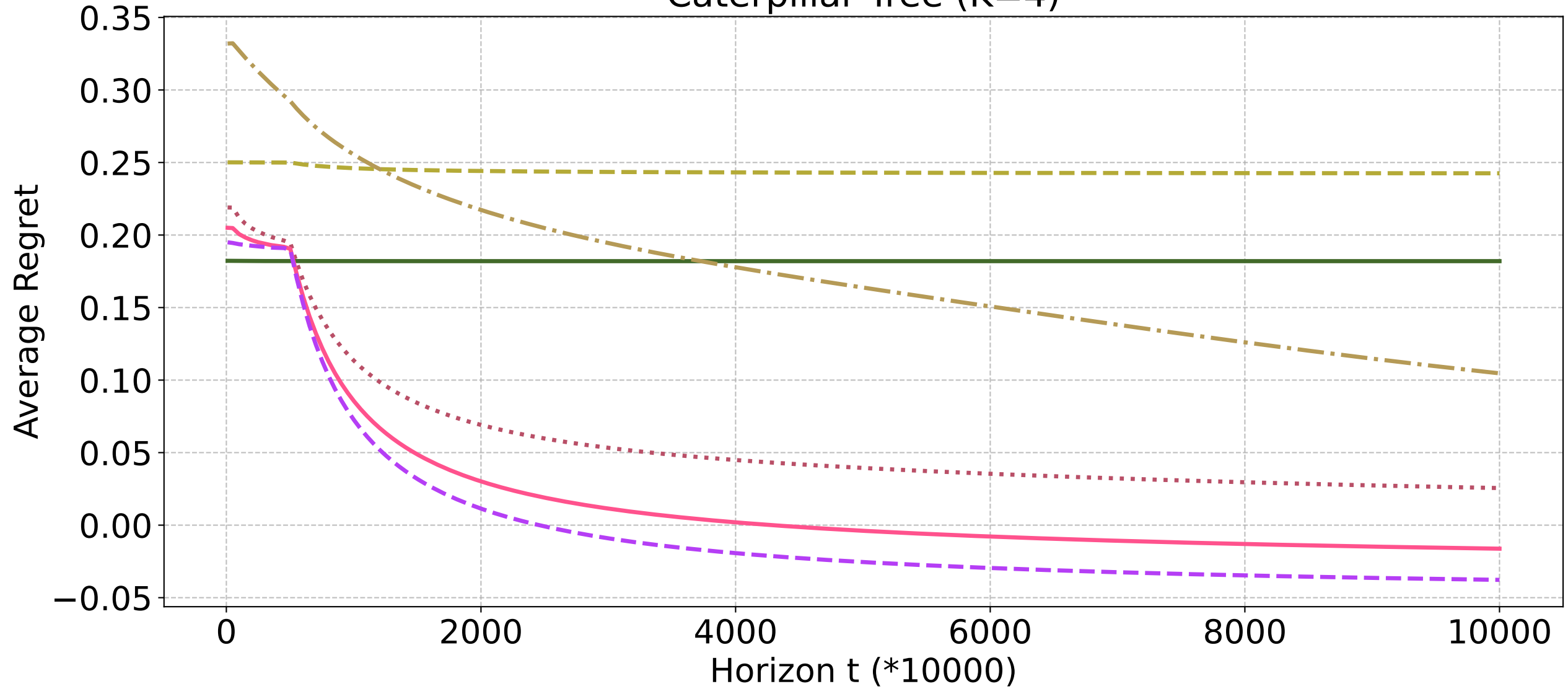
Caterpillar Tree (K=4)
