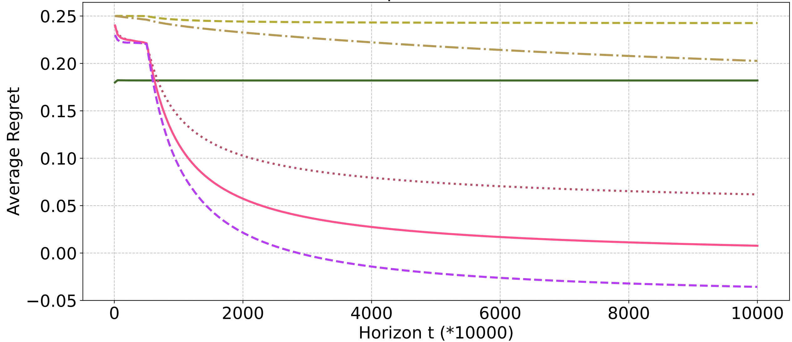
Caterpillar Tree (K=7)
