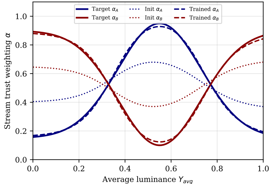
(a) ANFIS fit to synthetic target
