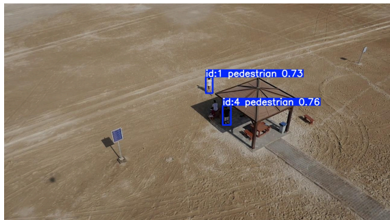
Edge (YOLOv26n) tracking post-occlusion of ID 1
