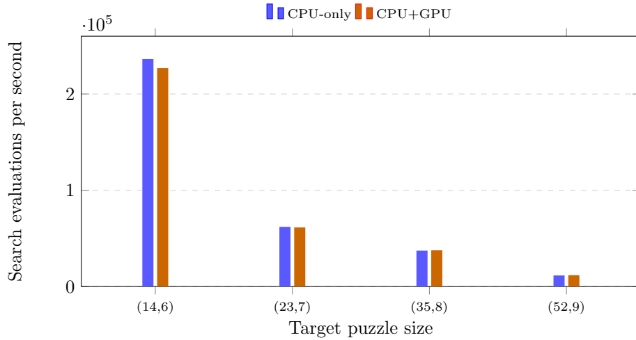
Fig. 1: End-to-end throughput of the original staged search program of Anderson and Le [4], with simplification forced to the CPU or with GPU simplification enabled.
