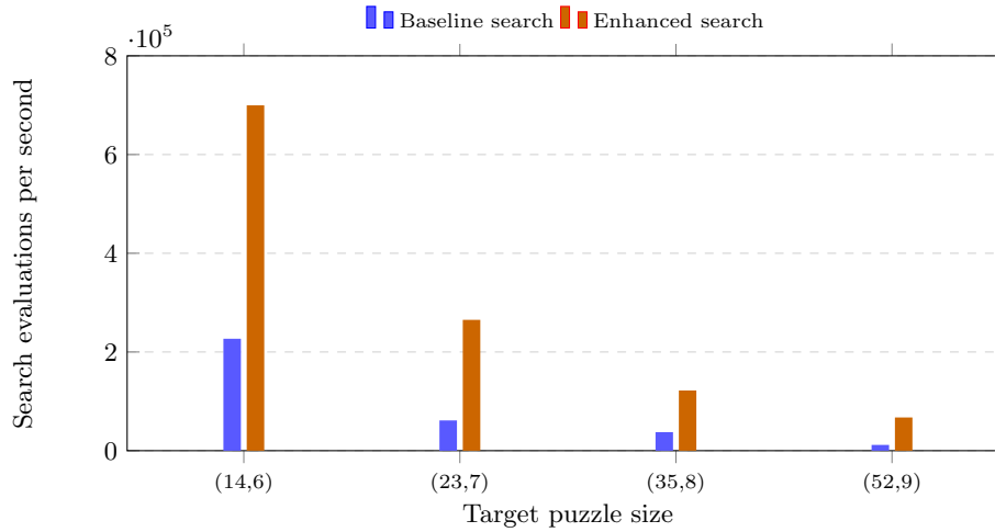
Fig. 8: End-to-end search evaluation throughput for the baseline staged search and the enhanced batched search.
