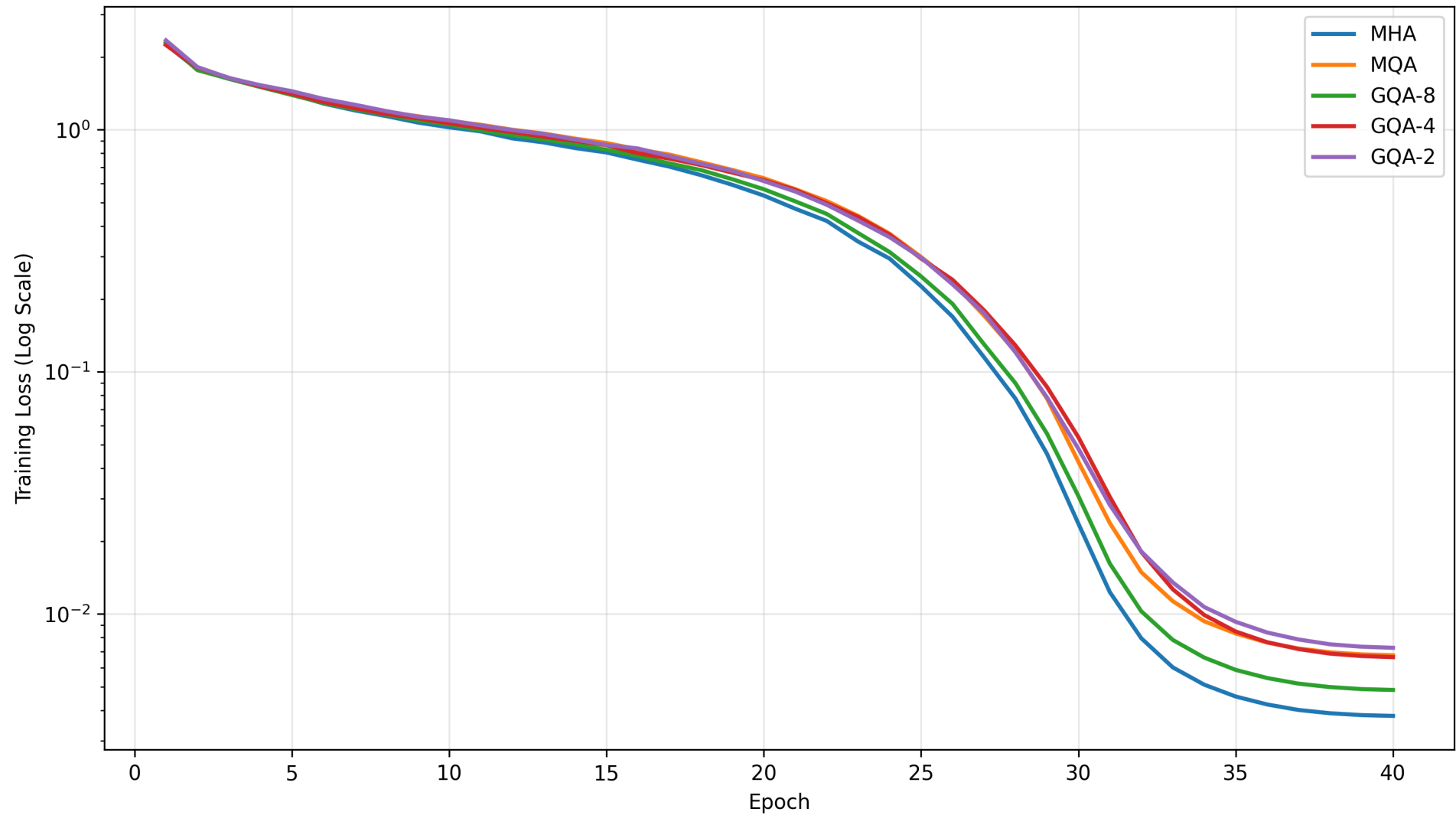
ViT Training Loss Comparison
