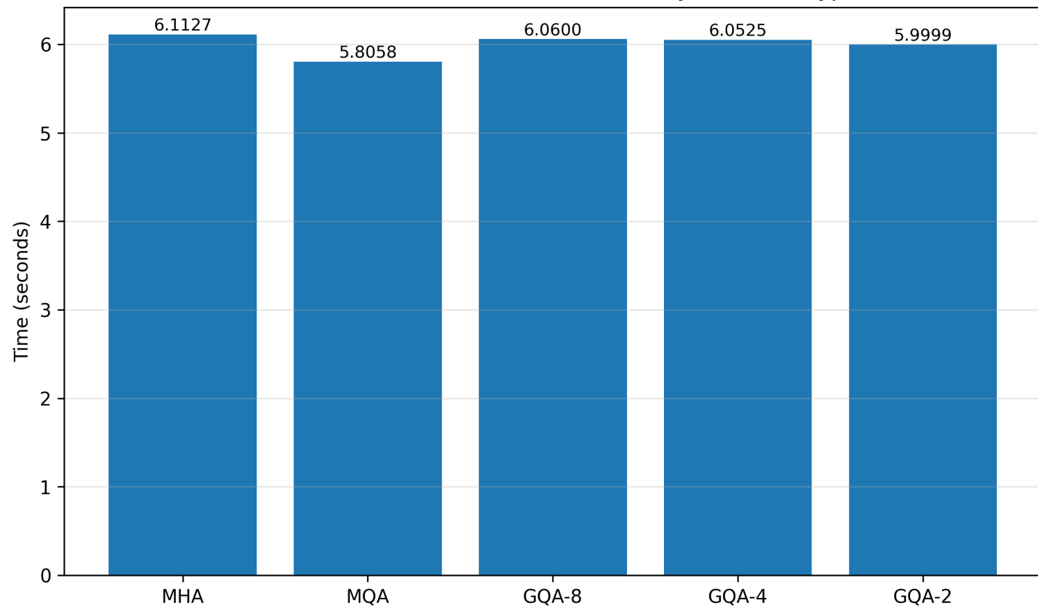
ViT Inference Time on CIFAR10 (Test) by Attention Type
