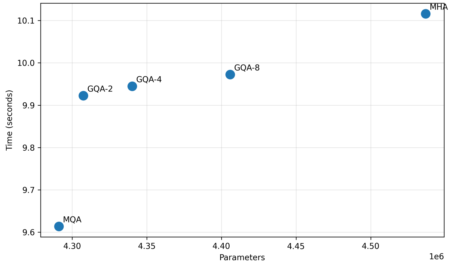
Conformer: Parameter Count vs Inference Time
