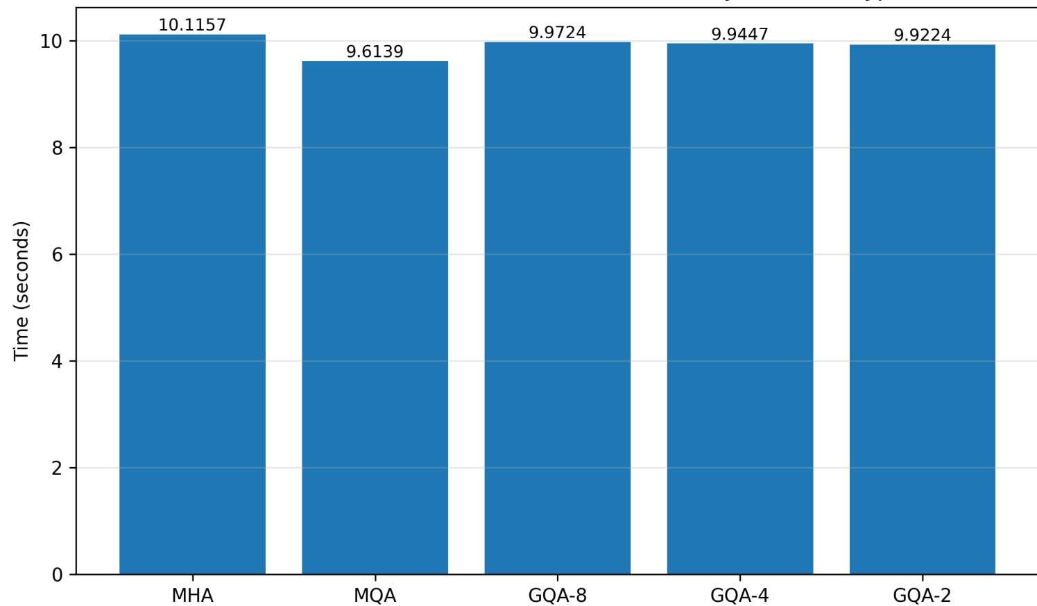
Conformer Inference Time on CIFAR10 (Test) by Attention Type
