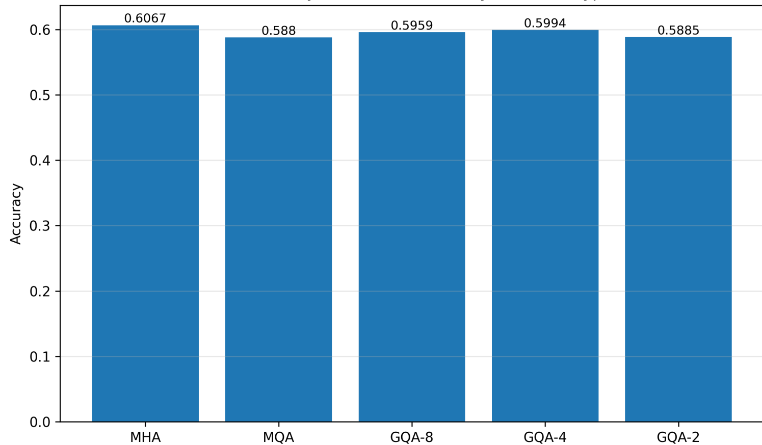
ViT Accuracy on CIFAR10 (Test) by Attention Type
