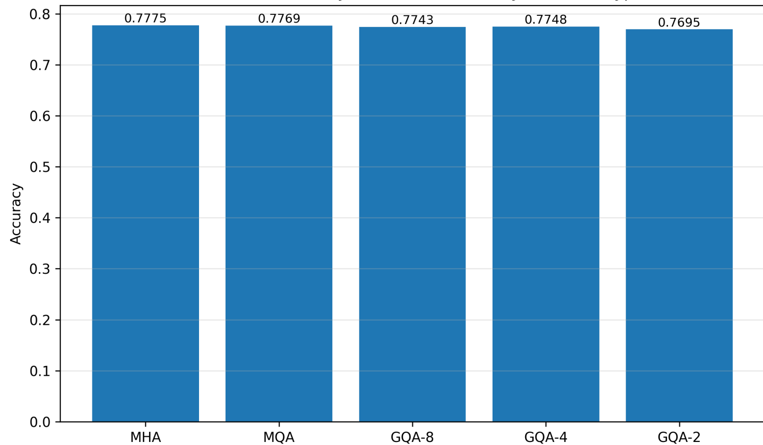
Conformer Accuracy on CIFAR10 (Test) by Attention Type
