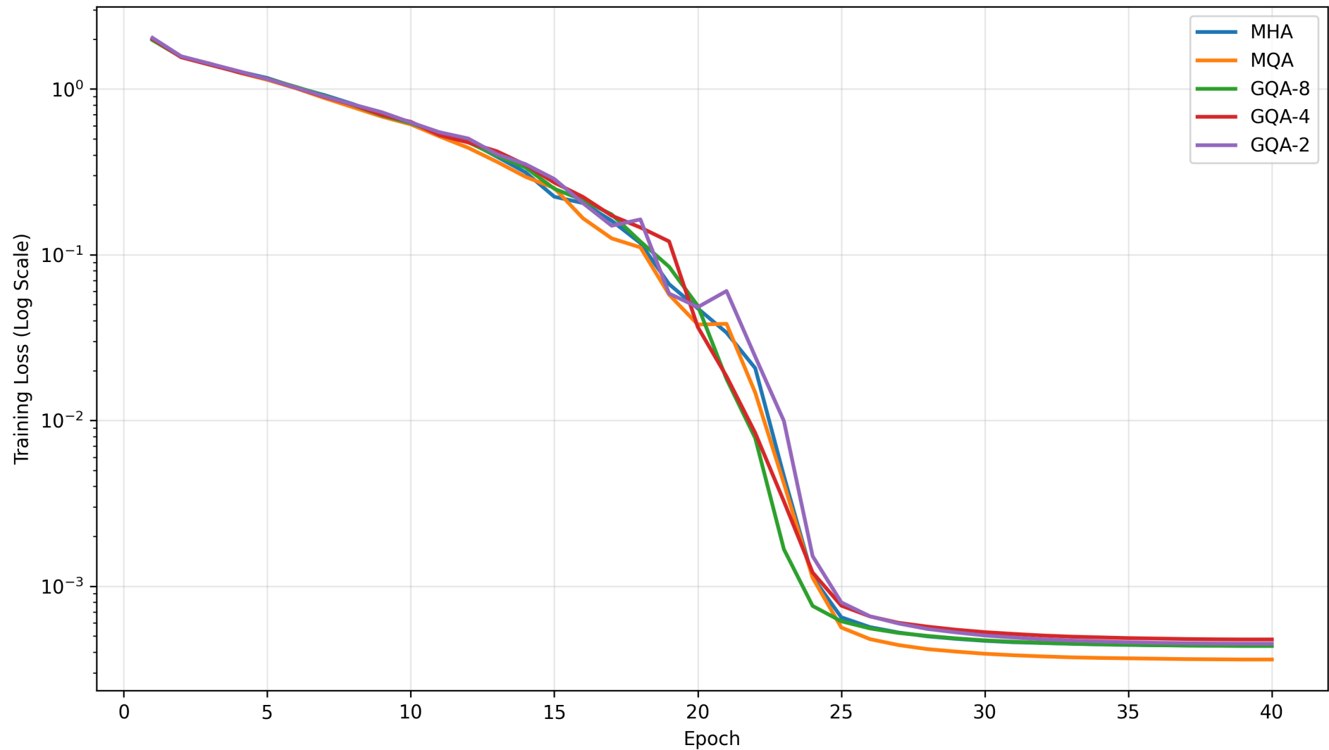
Conformer Training Loss Comparison
