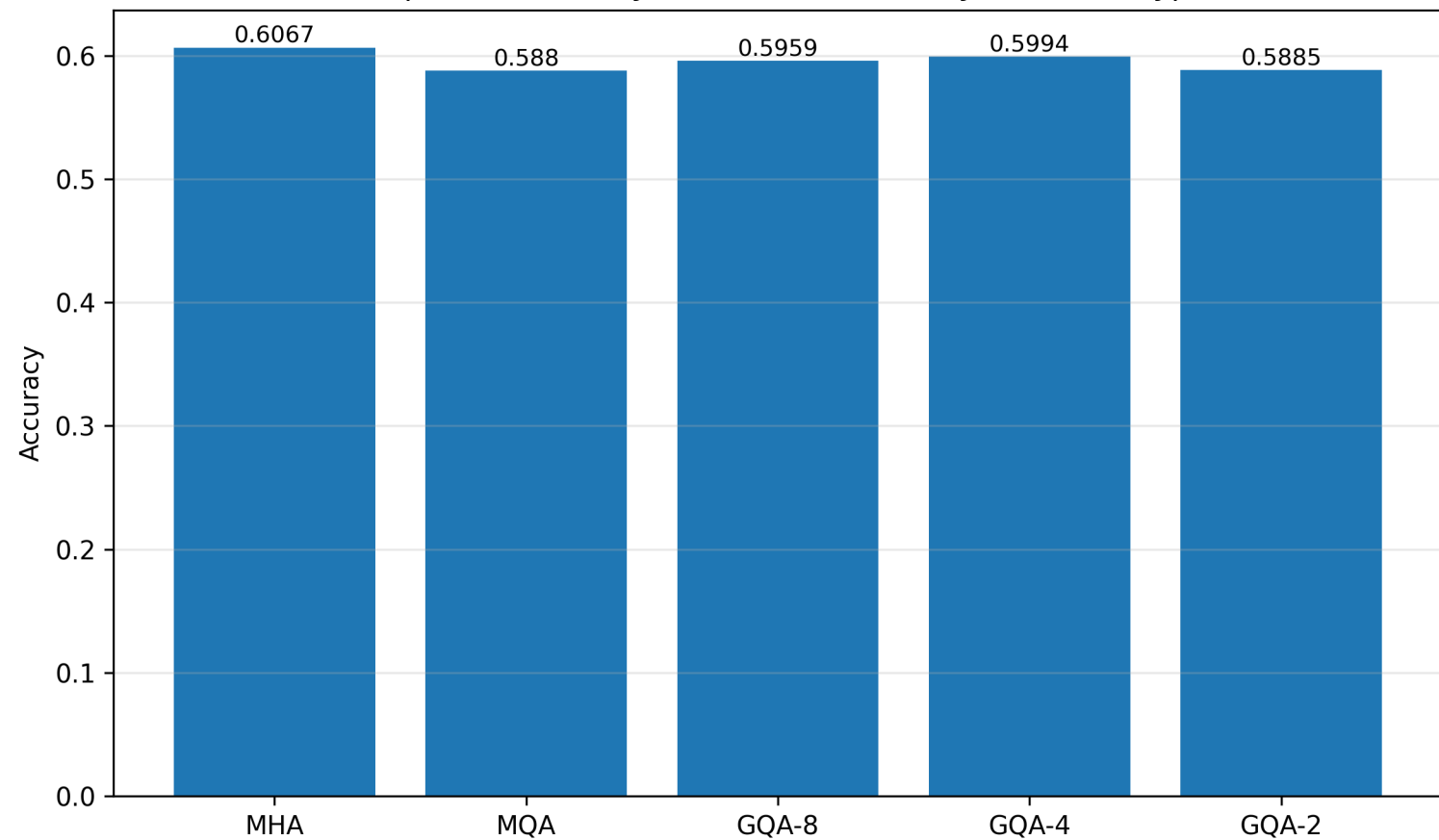
SimpleViT Accuracy on CIFAR10 (Test) by Attention Type
