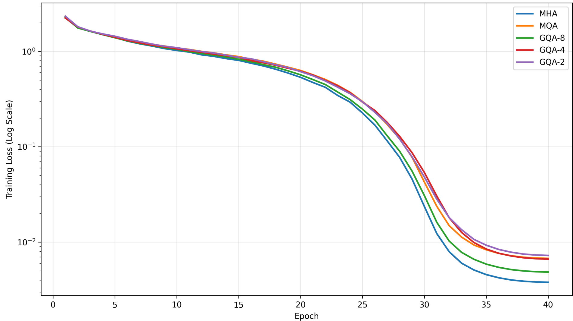
SimpleViT Training Loss Comparison
