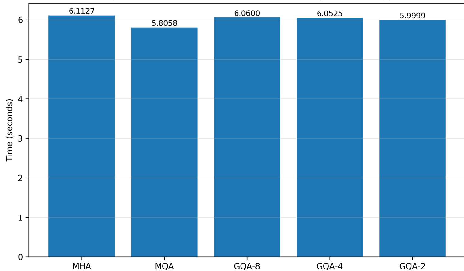
SimpleViT Inference Time on CIFAR10 (Test) by Attention Type
