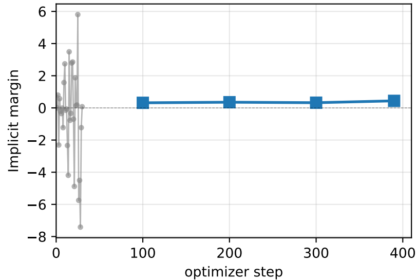
MQ training metrics: v3 picked recipe (windowed) vs v2 (per-step)
