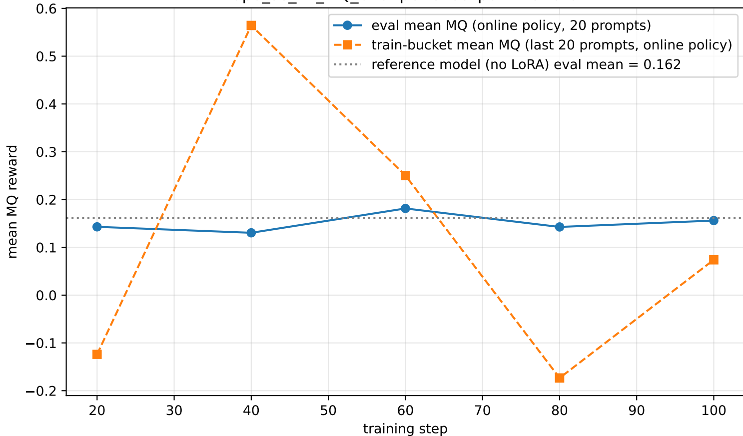
dpo_5s_v1_MQ_b10: per-checkpoint reward
