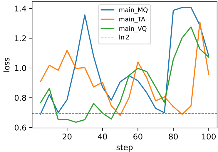
Loss EMA
