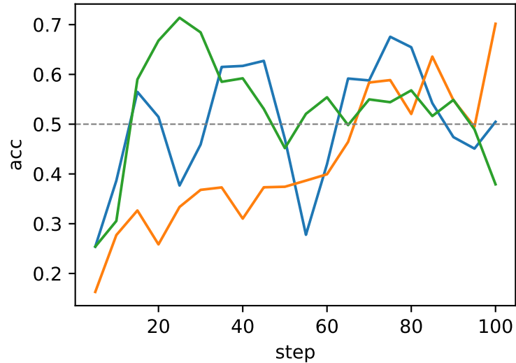
Accuracy EMA
