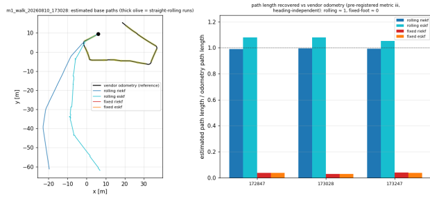
Fig. 2. Wheeled-legged M1, real rolling traverses. Left: estimated base paths against the vendor odometry (thick olive = the straight-rolling runs used for testing). Right: the heading-independent metric — fraction of the driven path length recovered. The rolling-contact model recovers essentially all of it; the fixed-foot model recovers almost none, because it treats a continuously rolling robot as near-stationary.
