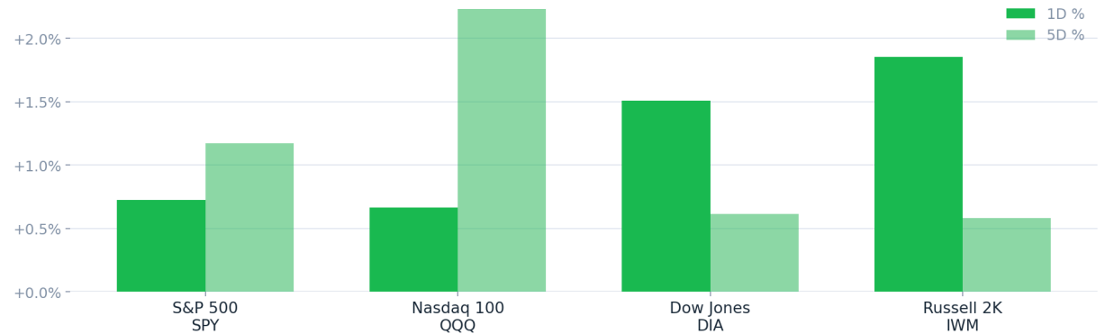
Index Returns — 1D vs 5D
