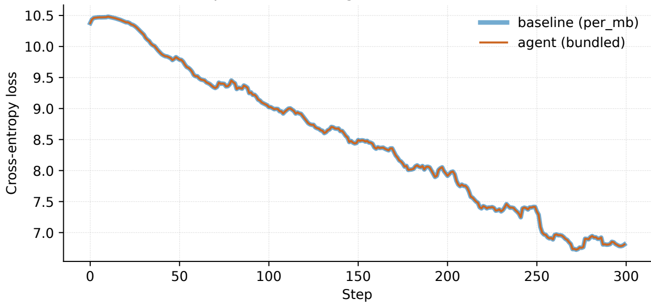
Llama-block real-OpenWebText, single-node TP=32, M=16 (bf16 AdamW)
