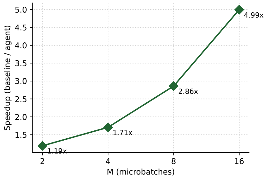
Speedup ratio
