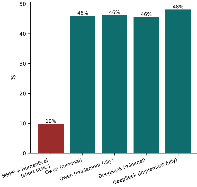
Share of generations carrying a defect
