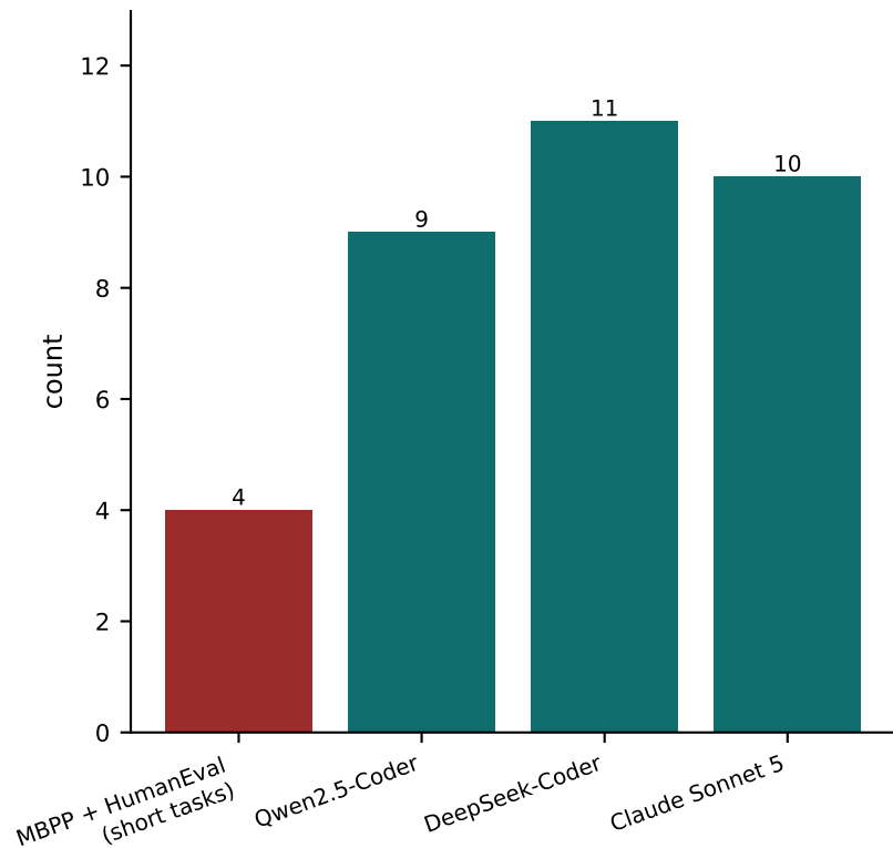
Distinct defects observed (of 12)
