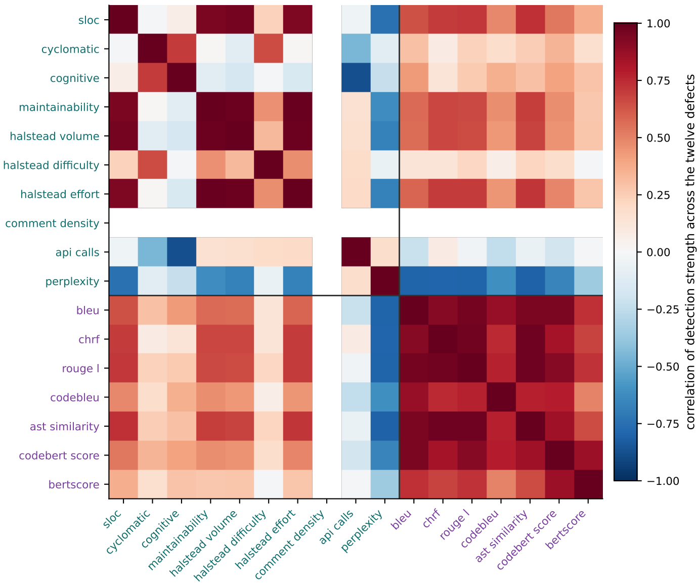
Measures that agree are redundant; the block structure is the empirical case for keeping both families
