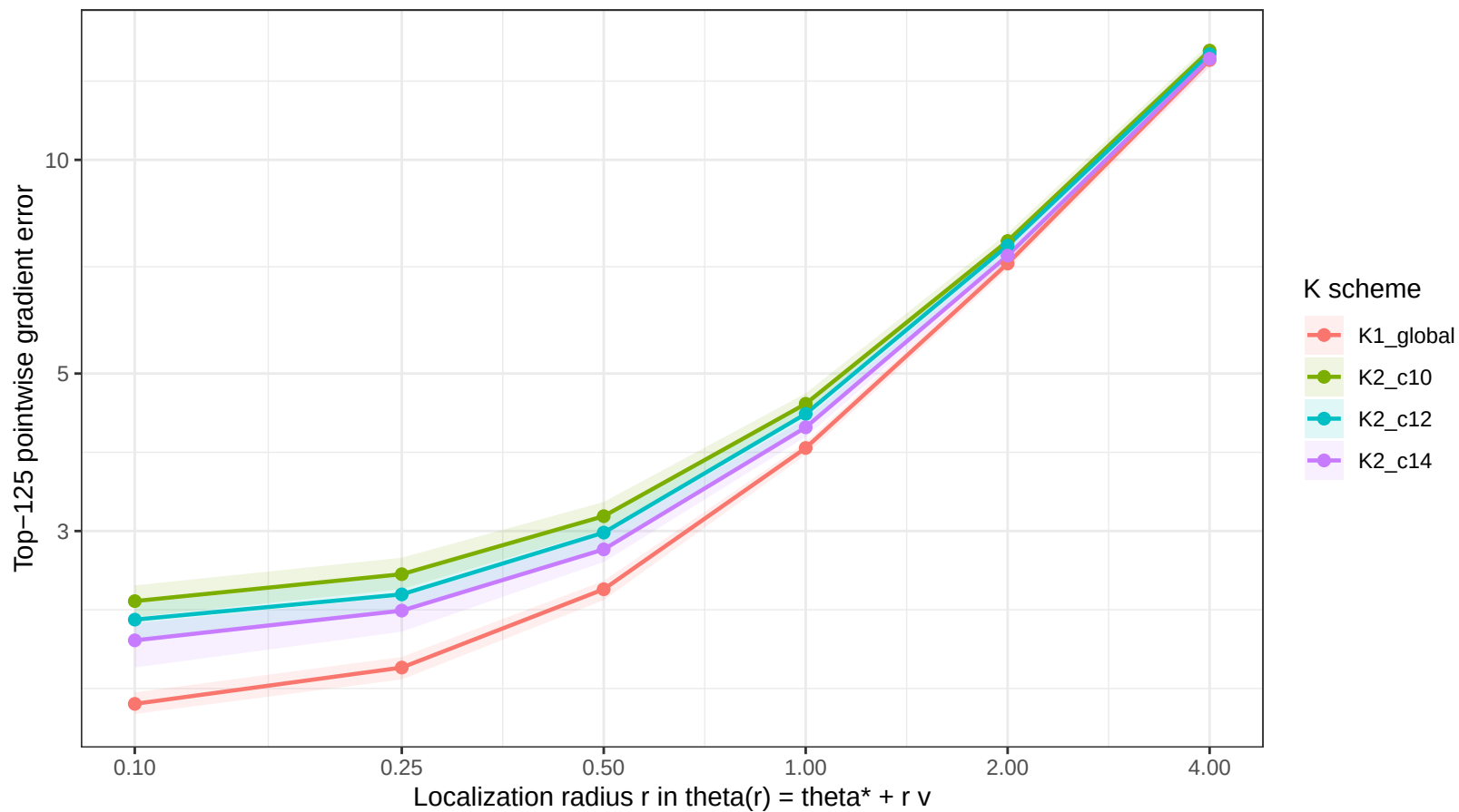
Linear pointwise gradient diagnostic with K2 constants
