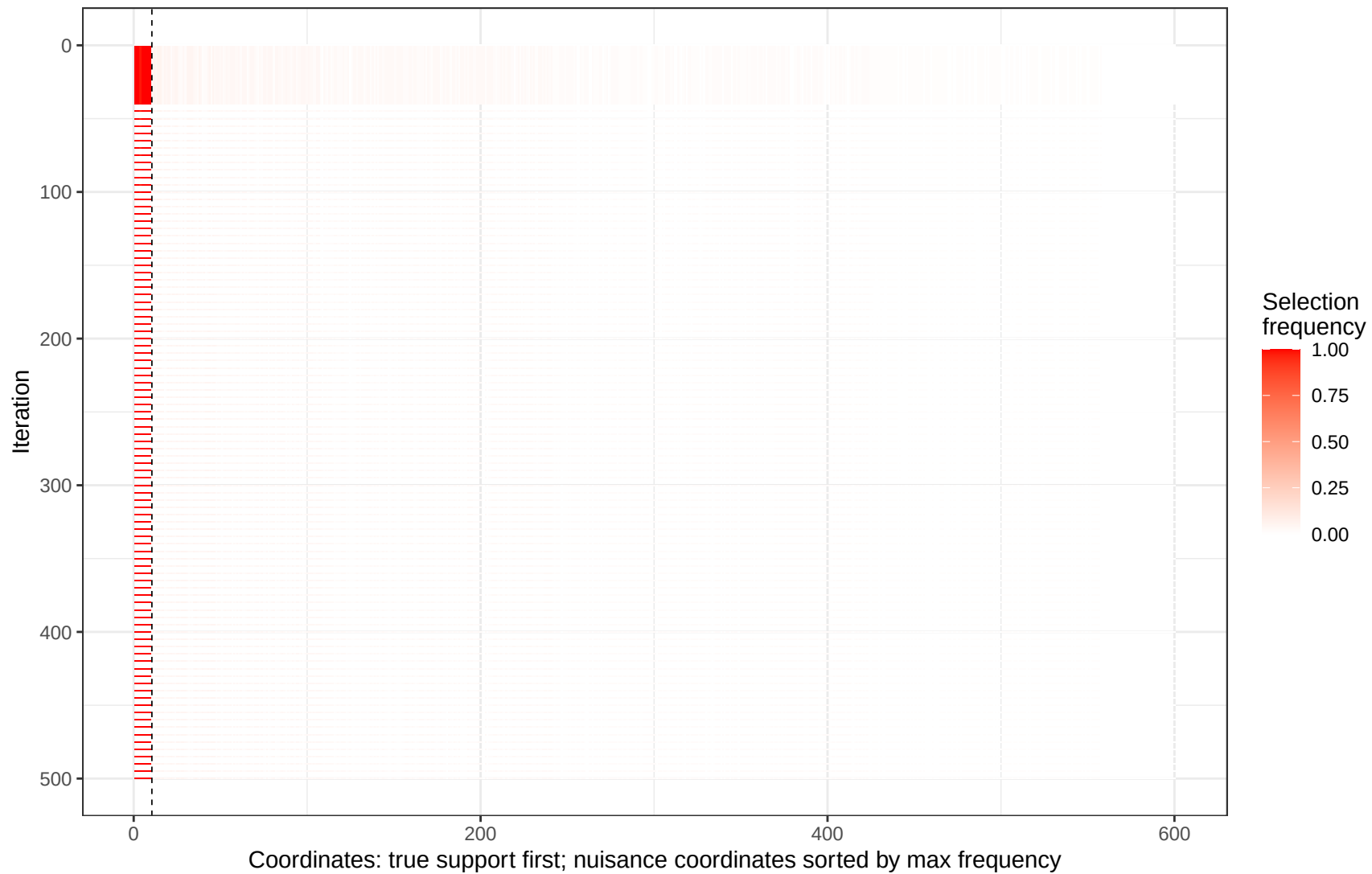
Linear FD-RIGHT empirical active-set diagnostic
