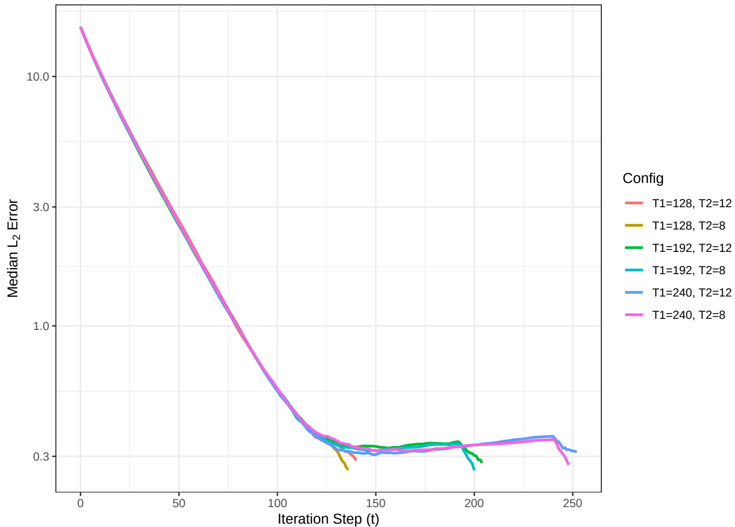
Median L2 Error Path over Iterations (100 Replications)
