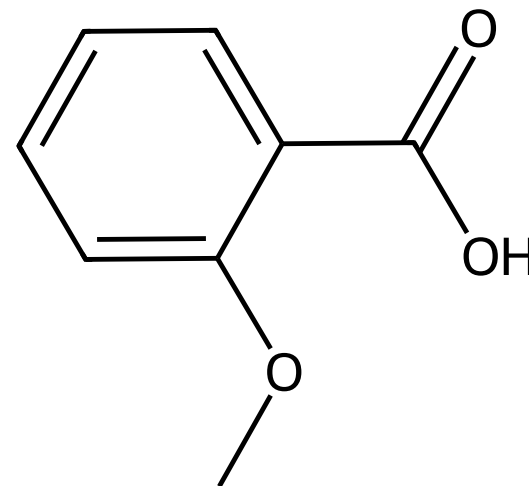
o -anisic acid
