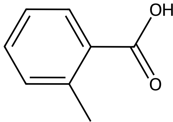
o -toluic acid
