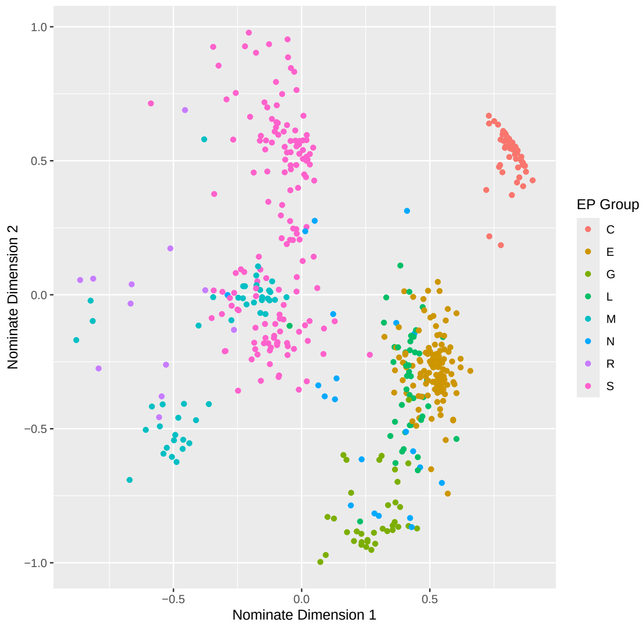
Scatterplot of Nominate Dimensions 1 and 2
