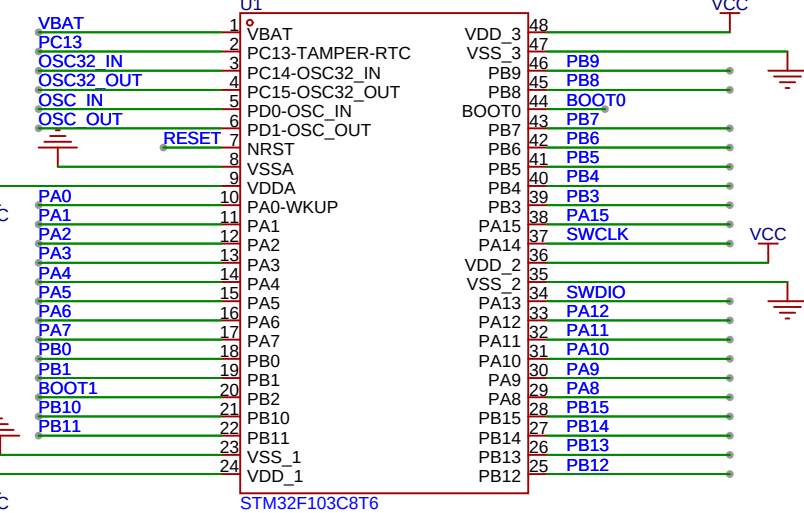
STM32F103C8T6
