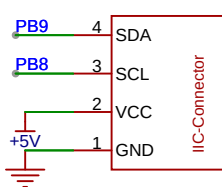
OLED
