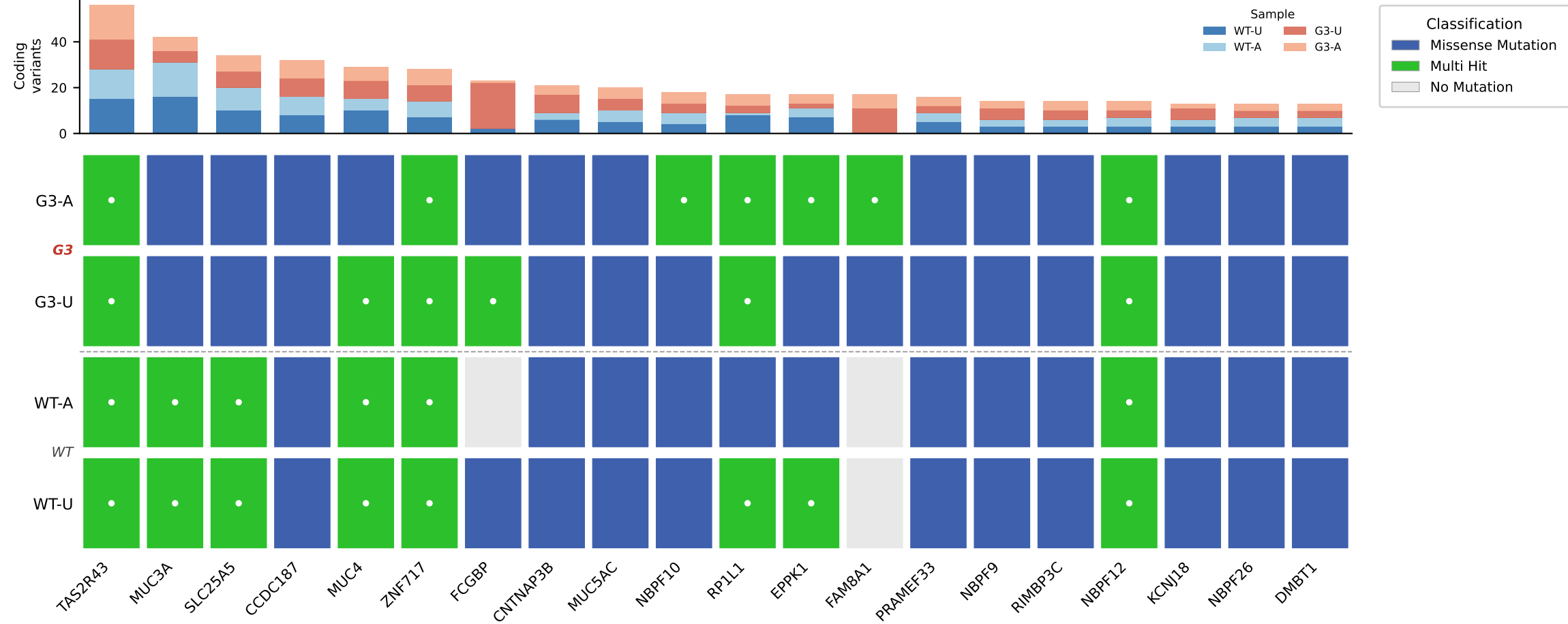
Top-20 mutated coding genes — U2OS
