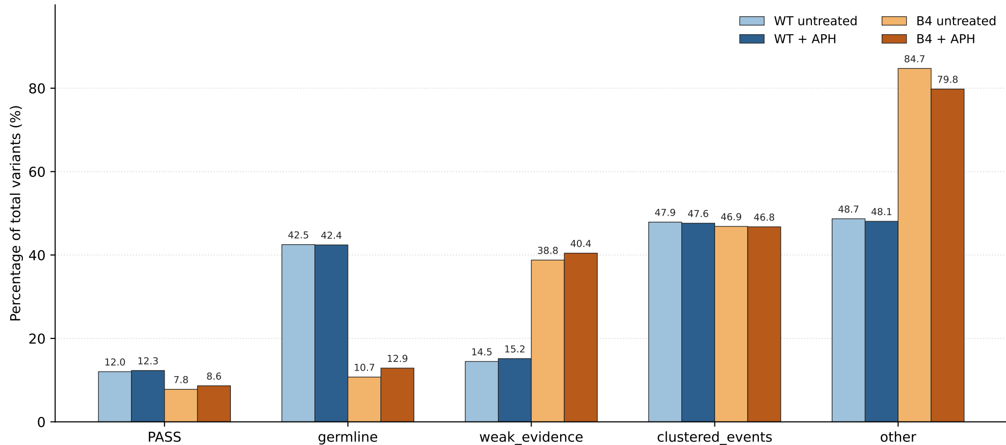
Filter-class prevalence per sample (percentage of total variants; classes may overlap)
