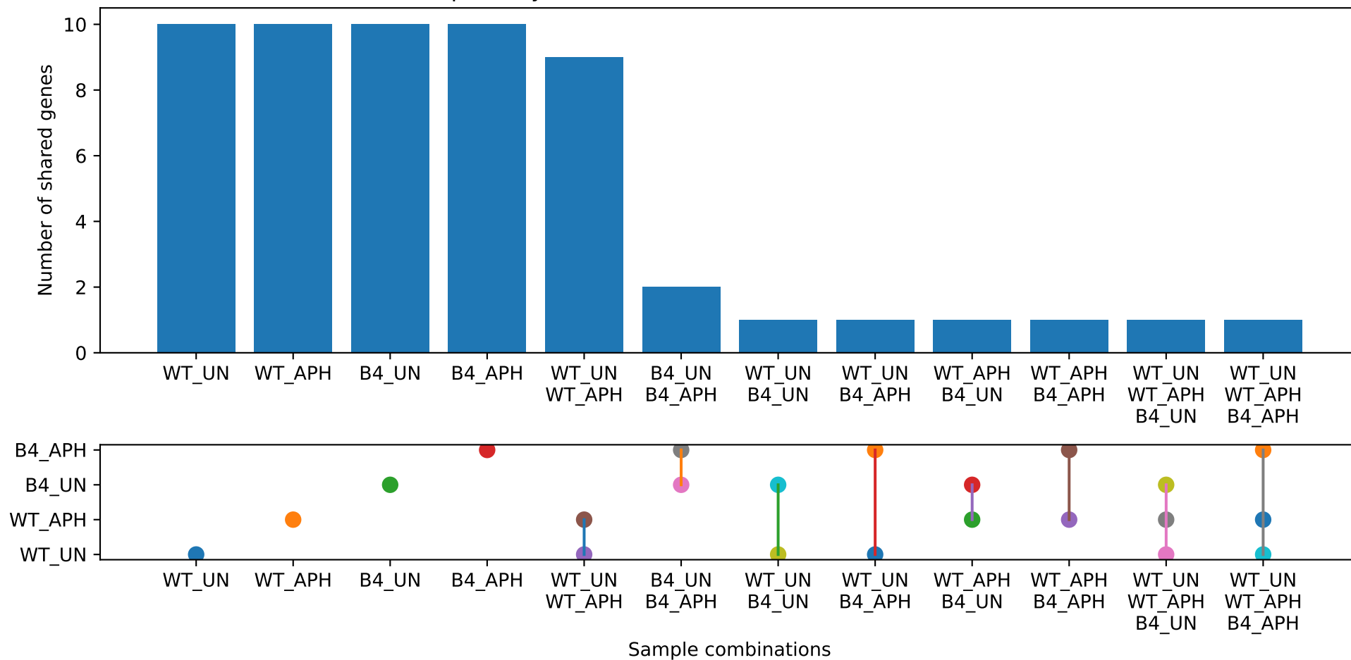
UpSet-style Intersection Plot of Most Mutated Genes
