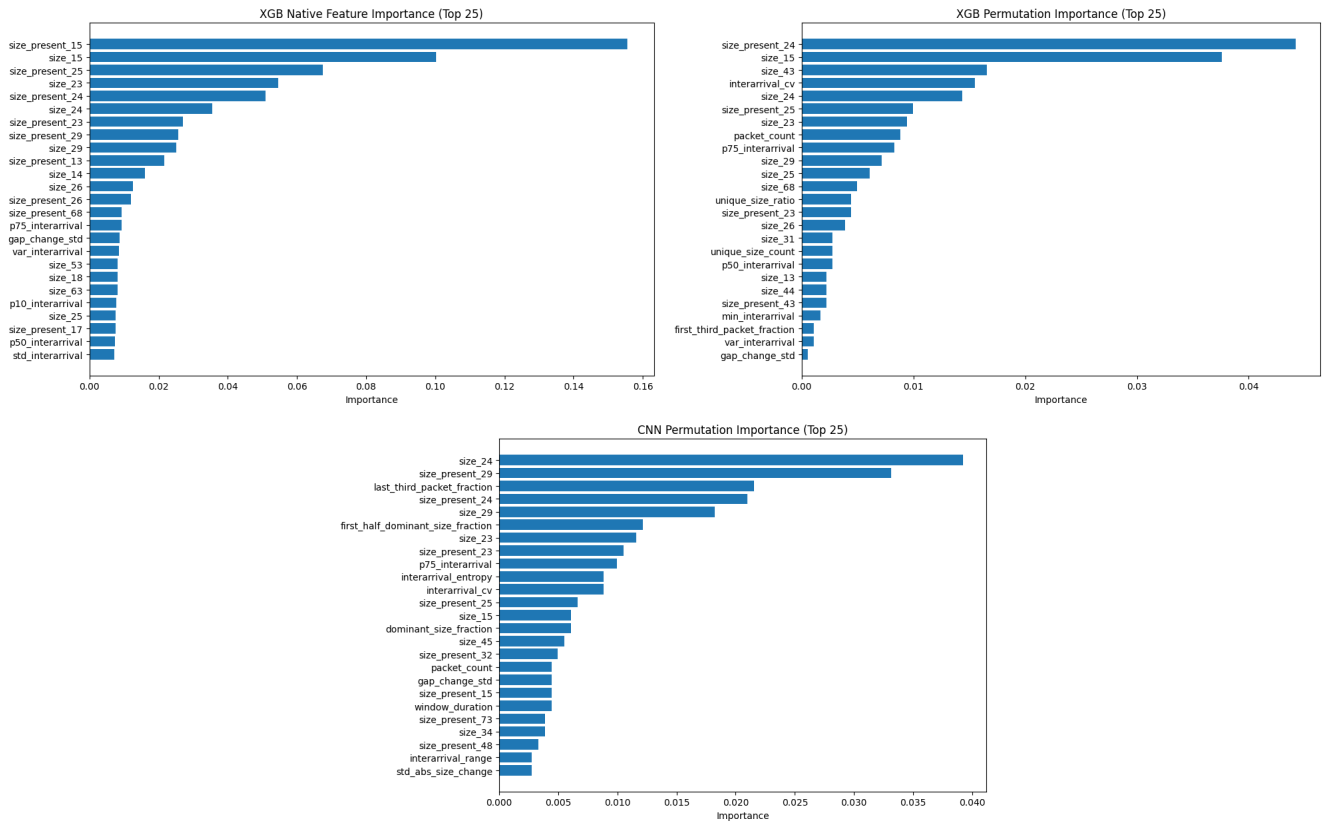
Fig. 10. Feature importance results for XGBoost and CNN.
