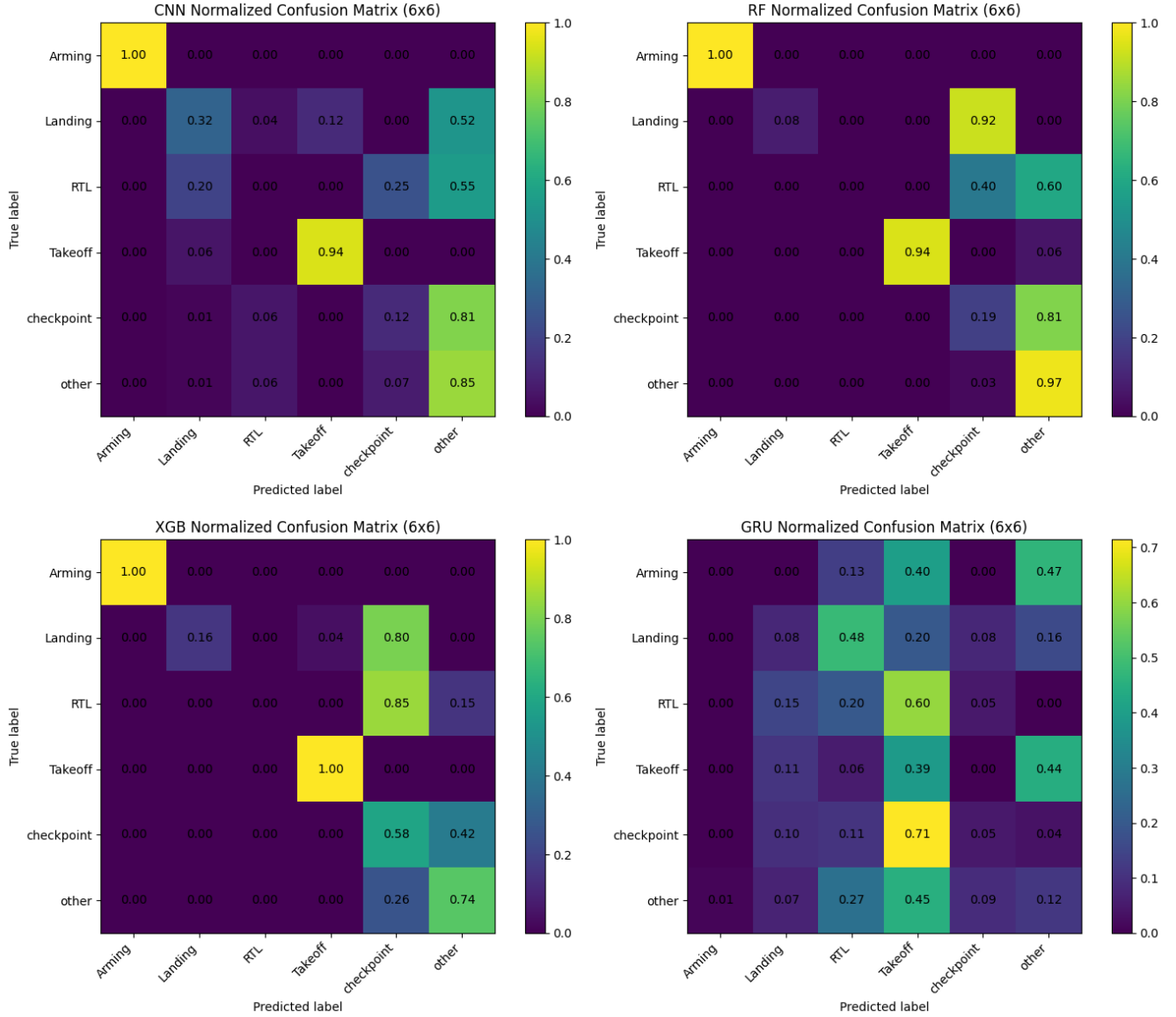
Fig. 9. Normalized confusion matrices for CNN, Random Forest, XGBoost, and GRU.
