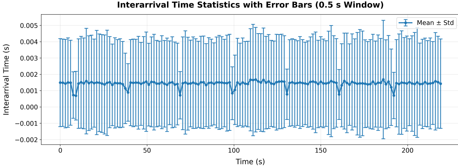
Fig. 7. Interarrival time statistics computed over sliding windows.
