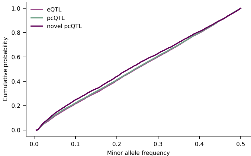
Allele frequency of pcQTL and eQTL lead variants
