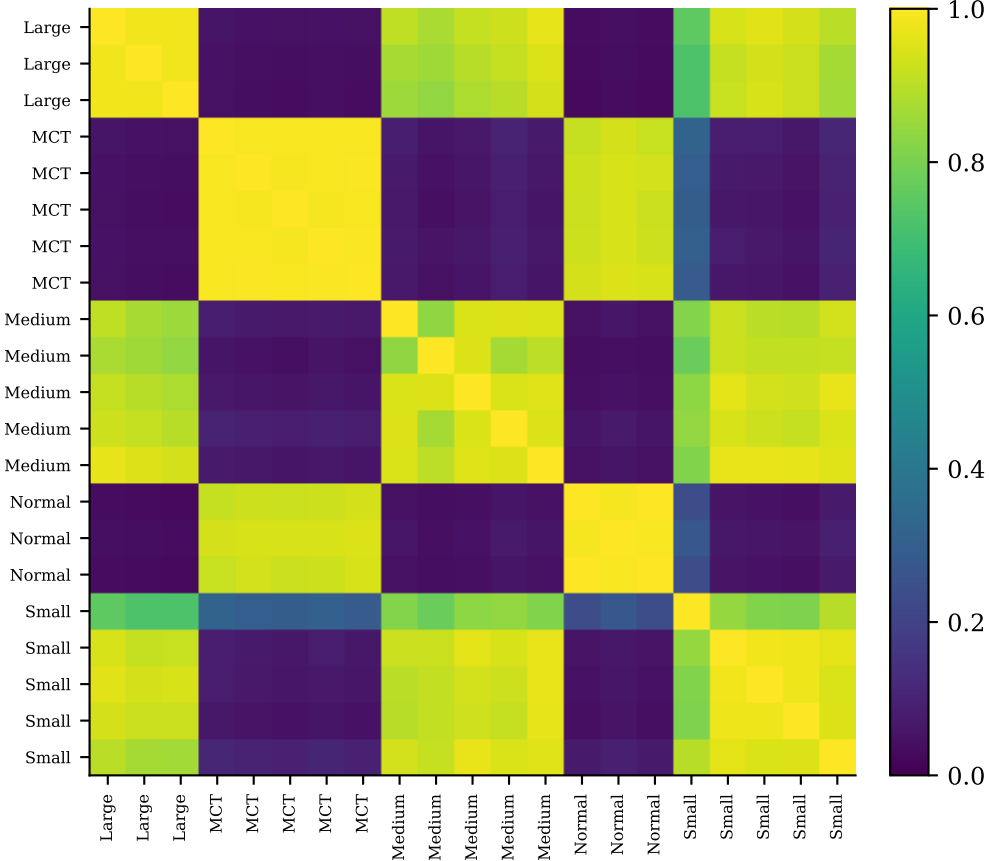
Quantum kernel (amplitude-embedding fidelity)
