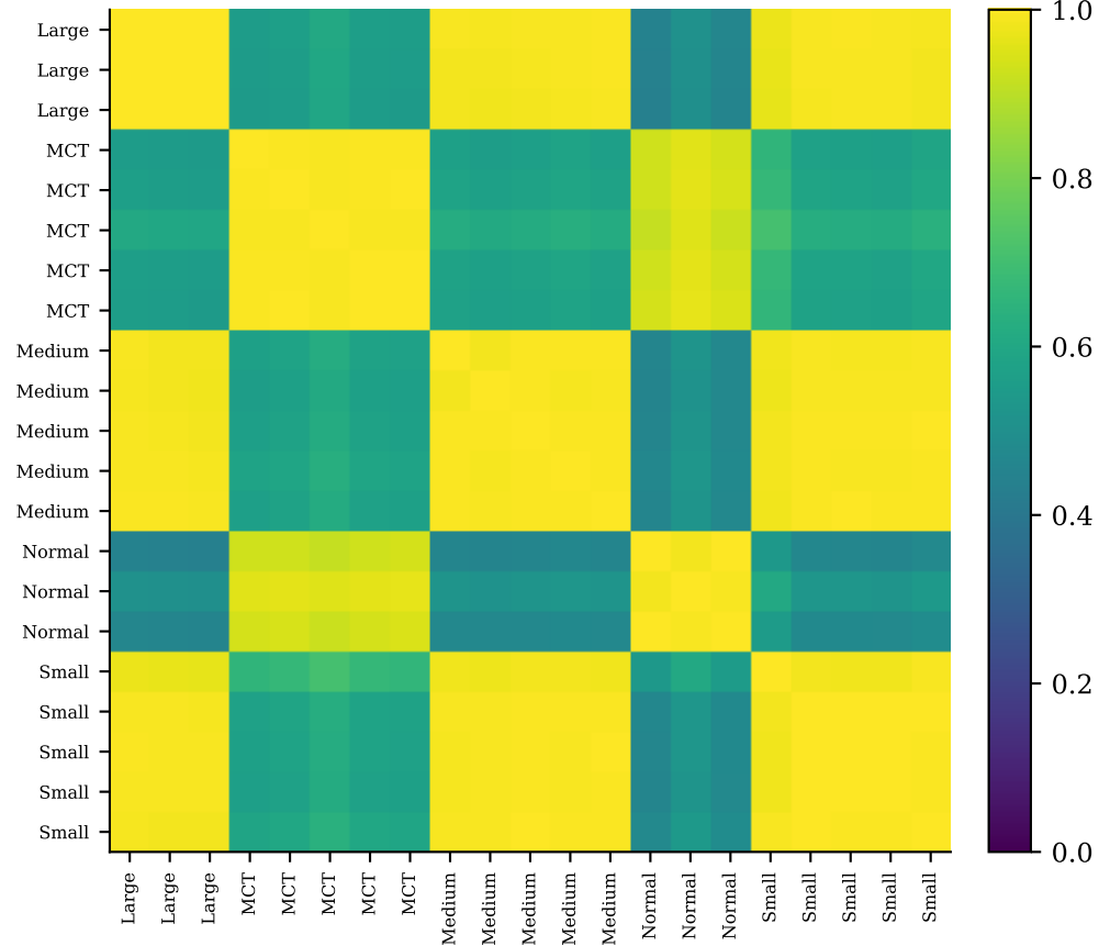
Classical RBF kernel
