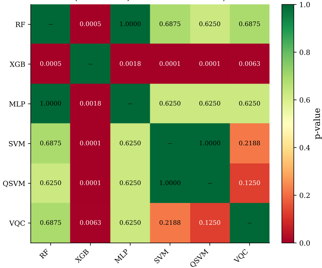
Pairwise exact McNemar p-values (six models, n=21 LOOCV folds)
