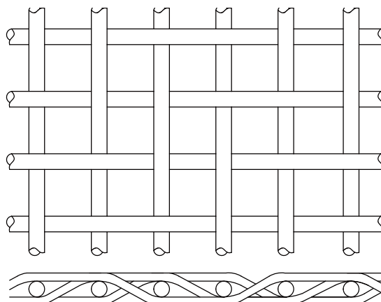
Twill weave
